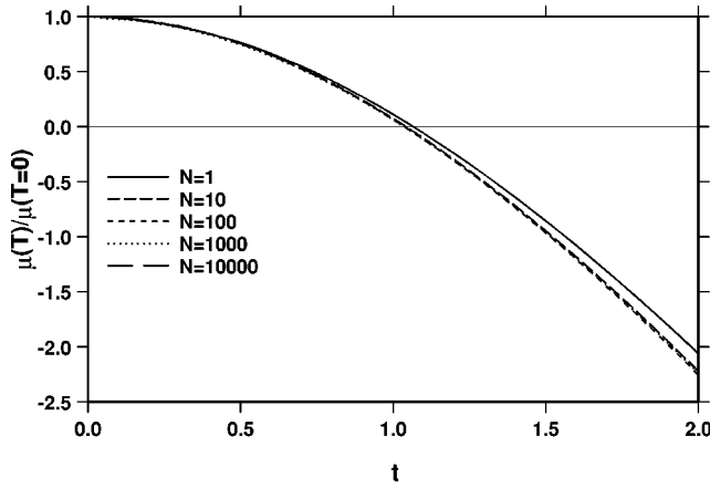
FIG. 1. Scaled chemical potential \mu(T)/\mu(T=0) as a function of the scaled temperature t = kT/\hbar\omega N^{1/3} for 10, 100, 1000, and 10 000 fermions. For reference, this quantity is also plotted for one particle.
